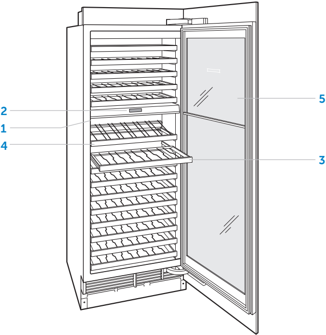
Column model
