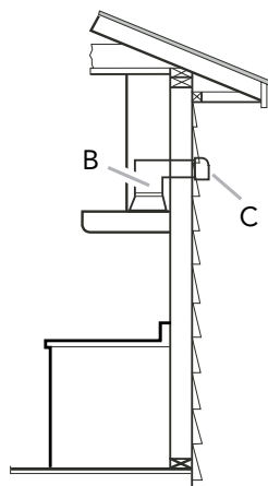
VENTING THROUGH THE WALL
