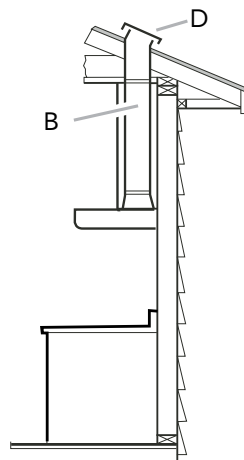
VENTING THROUGH THE CEILING
