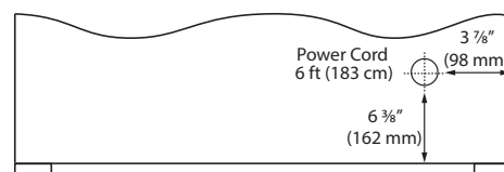
Cabinet Cut-Out
