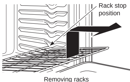
Removing racks
