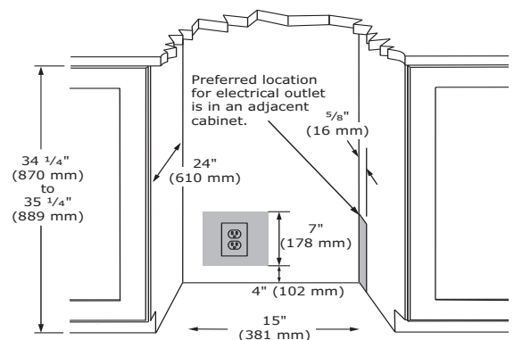
Cabinet Cut-Out
