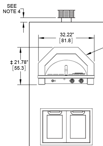
SECTION VIEW
