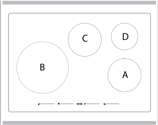
30" Wide Cooktop. Use the minimum size pan shown for each cooking element.
