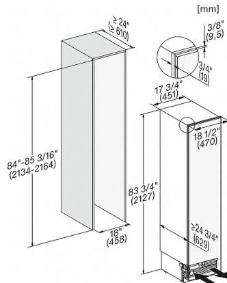
F2412SF, F2411SF, MasterCool, inner space, installation drawings
