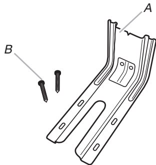
A. Anti-tip bracket B. #12 x 1½" (4.1 cm) screws (2)
