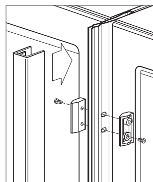
Clip installation.
