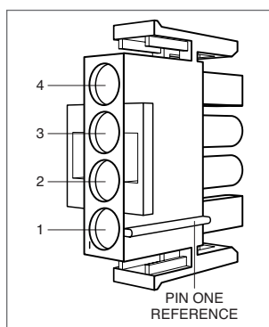
Pin placement.
