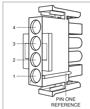
Pin placement.
