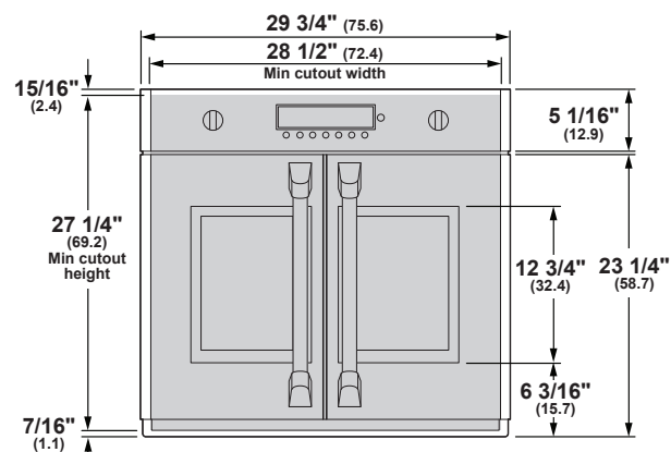
FRONT VIEW (SHOWING CUTOUT OVERLAP)
