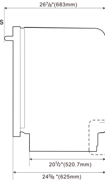
Side view DW80R2031 Series
