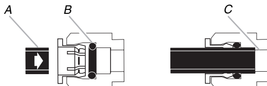
A. 1/4" water supply tubing B. O-ring C. Backstop
