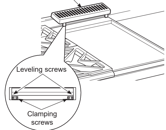
Griddle flue cover
