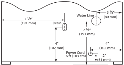
Cabinet Cut-Out
