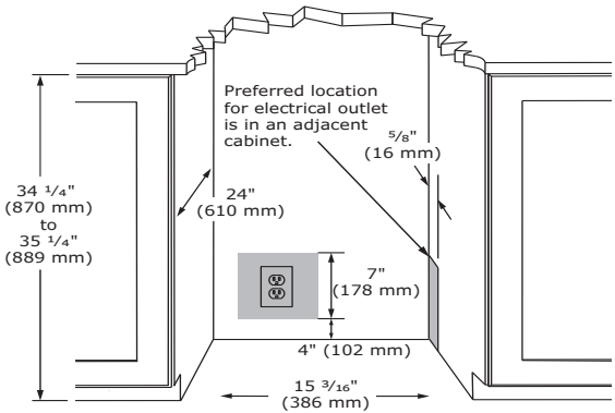
Cabinet Cut-Out
