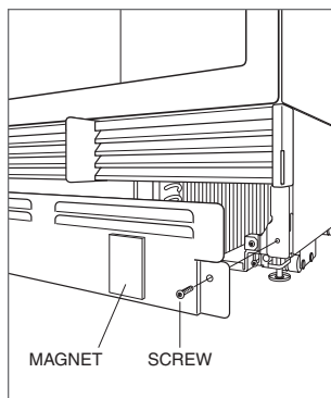
Kickplate installation.
