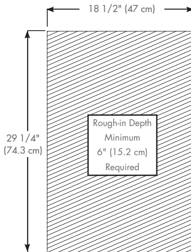
Rough-in Dimensions
