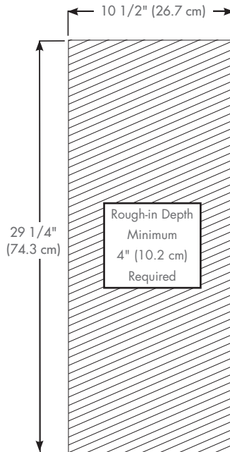
Rough-in Dimensions
