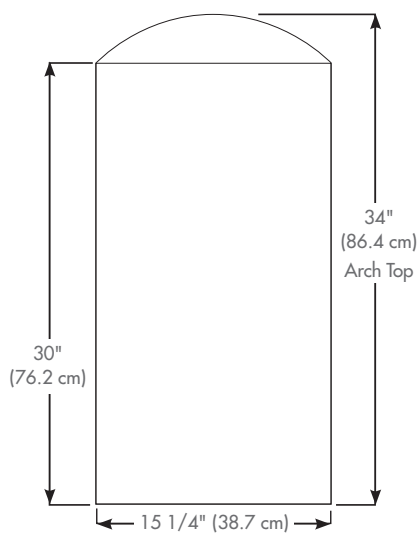
Cabinet Dimensions
