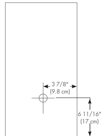
Back of Cabinet - Wire Access Location
