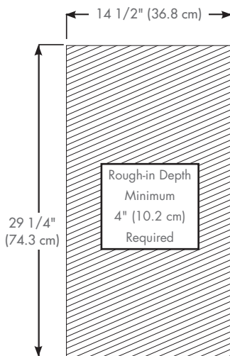
Rough-in Dimensions
