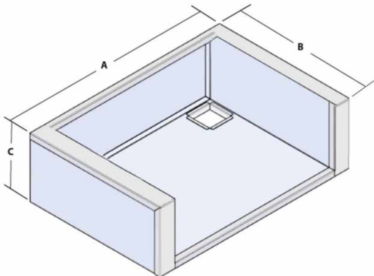
INSULATED JACKET DIMENSIONS (INCHES)
