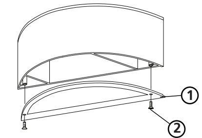
Drawing 2 - Fixture Assembly
