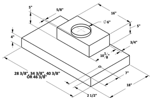
290 CFM MODELS
