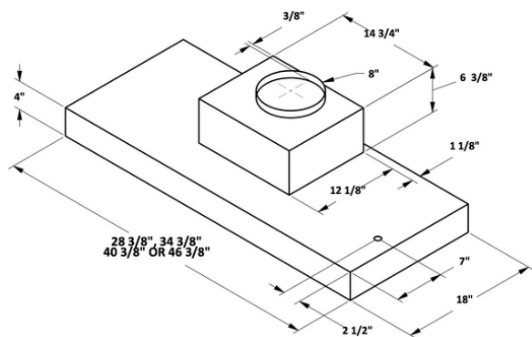
600 CFM MODELS
