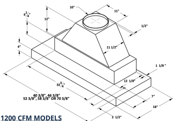
1200 CFM MODELS
