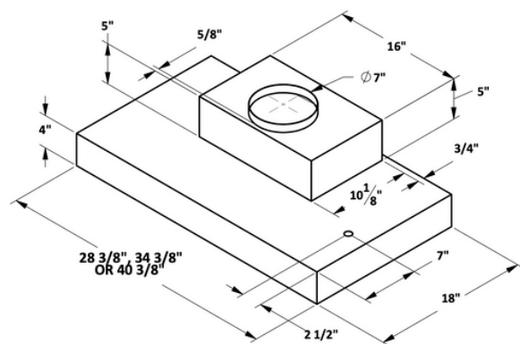
390 CFM MODELS
