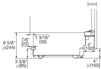
Side-by-side, MasterCool, without partition wall, with heating mat (Sketch) (with footnote)
