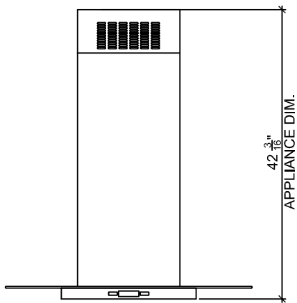
2 FRONT ELEVATION
