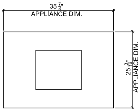
1 PLAN
