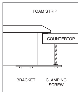
Cooktop installation
