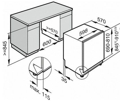
G2000/G2002 fully integrated dishwashers (installation drawing)
