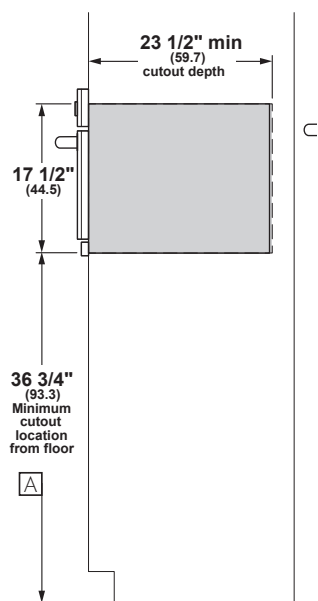
STANDARD INSTALLATION
