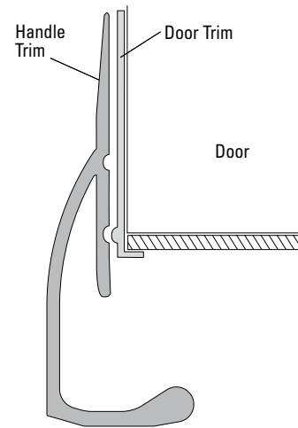
Standard supplied handle shown in 1/4" panel position.
