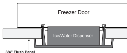
3/4" OVERLAY PANEL DISPENSER TRIM
