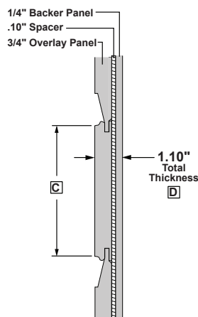
SIDE VIEW CROSS SECTION (SHOWING RAISED OVERLAY WITH MIDDLE RAIL)
