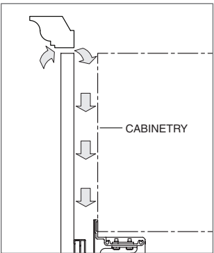
Air flow above grille panel
