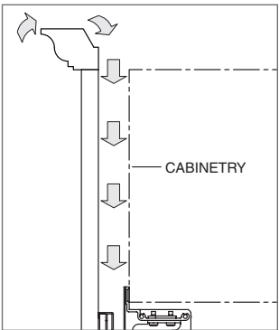
Air flow above molding
