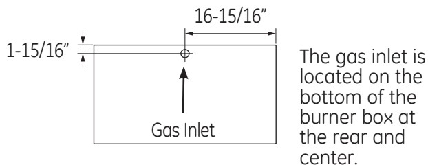
Rear-Burner Box
