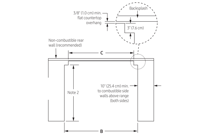
CUTOUT WITH OPTIONAL DOWNDRAFT VENT TOP VIEW
