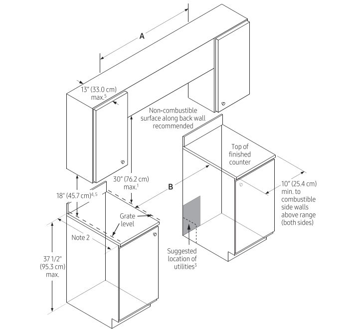
STANDARD CUTOUT WITH RANGE HOOD
