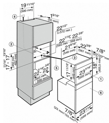
DGC 6000 XL in a tall unit with oven (Installation drawing) - USA
