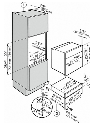
ESW 6114, ESW 6214 with H 6xxx B(P), Hxxx B(P) 60 cm high (Installation drawing) - USA
