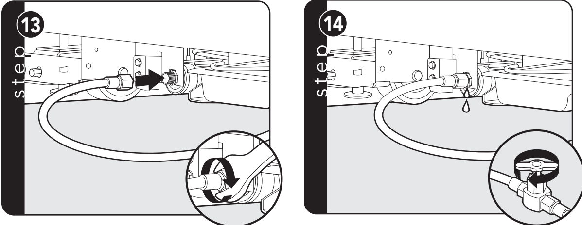
Connect supply tube to water valve using a 1/2" wrench. NOTE: DO NOT overtighten. Turn on water supply and check for leaks.
