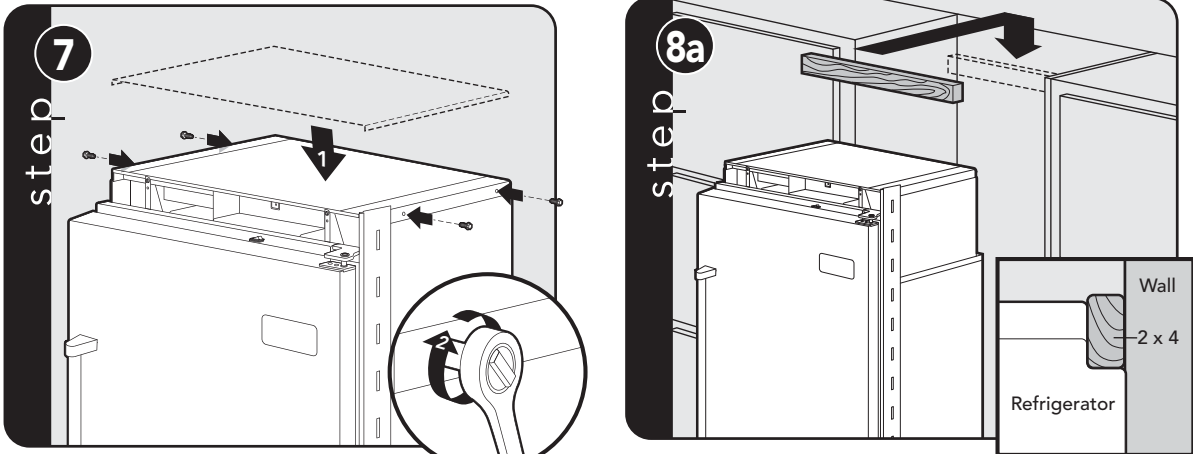
Replace unit top. Replace four side screws. Attach one 2x4 to wall stud (refer to dimensions page for exact location).
