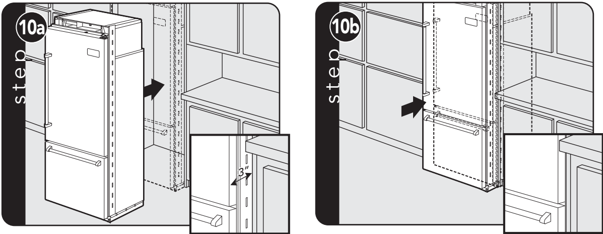
Place unit within 3" of being flush with cabinets. NOTE: To avoid cabinet damage, place cardboard between cabinets and unit. When moving unit, do not crimp, kink or crush water supply line.
