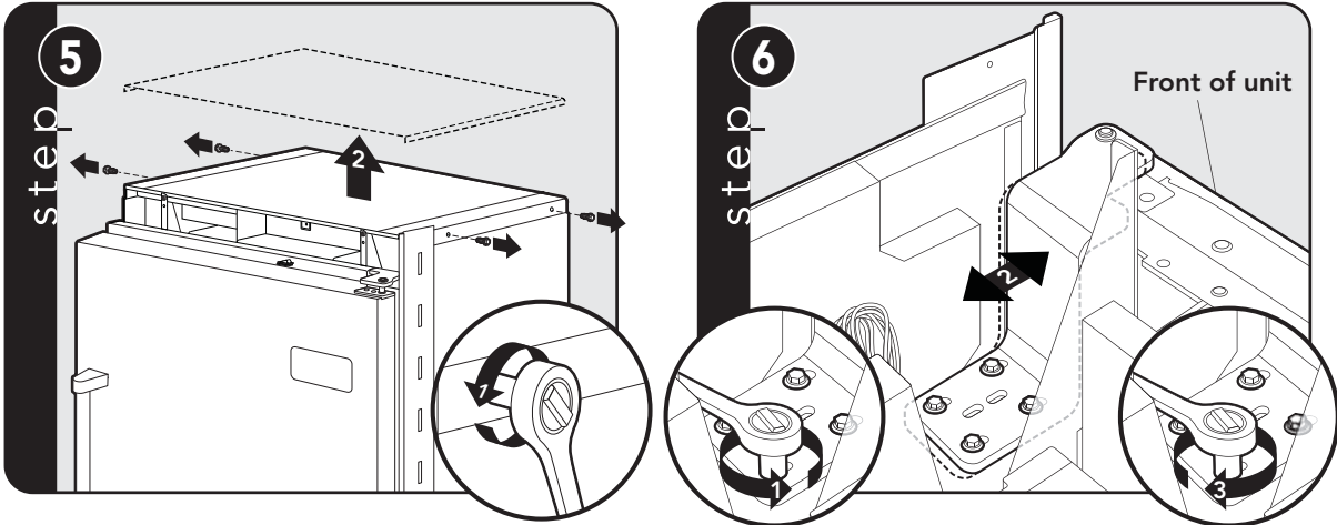
Remove four side screws and remove unit top. Loosen the four hinge screws. Adjust door. Retighten four hinge screws.
