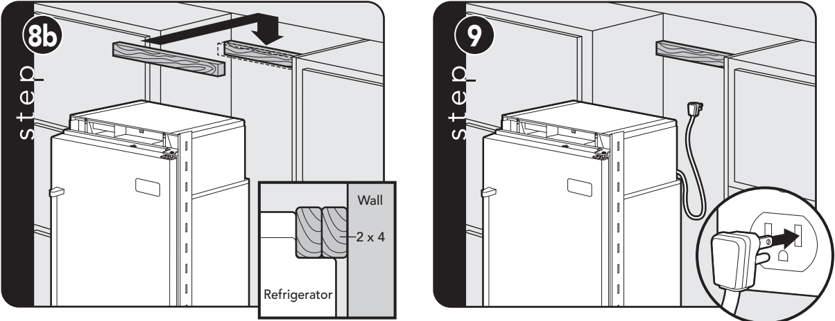
If needed, depending on cabinet and depth, attach second 2x4 to first 2x4. Plug in power cord to verify operation. NOTE: Make sure power switch is in the "On" Position.
